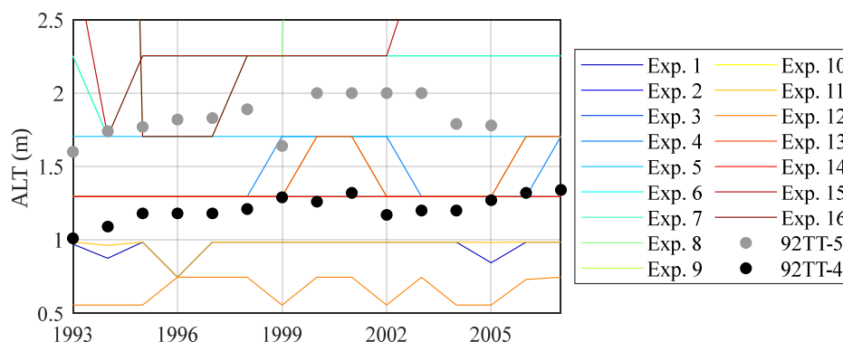
415 Fig. 7. Simulated and observed ALT for Manners Creek sites (92TT-5 and 92TT-4) for the needleleaf forest GRU.
