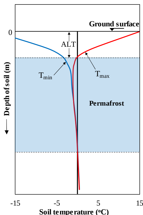
Fig. 2. Schematic of the soil column showing variables used to represent permafrost dynamics, modified after Abdelhamed et al. (2022a).
