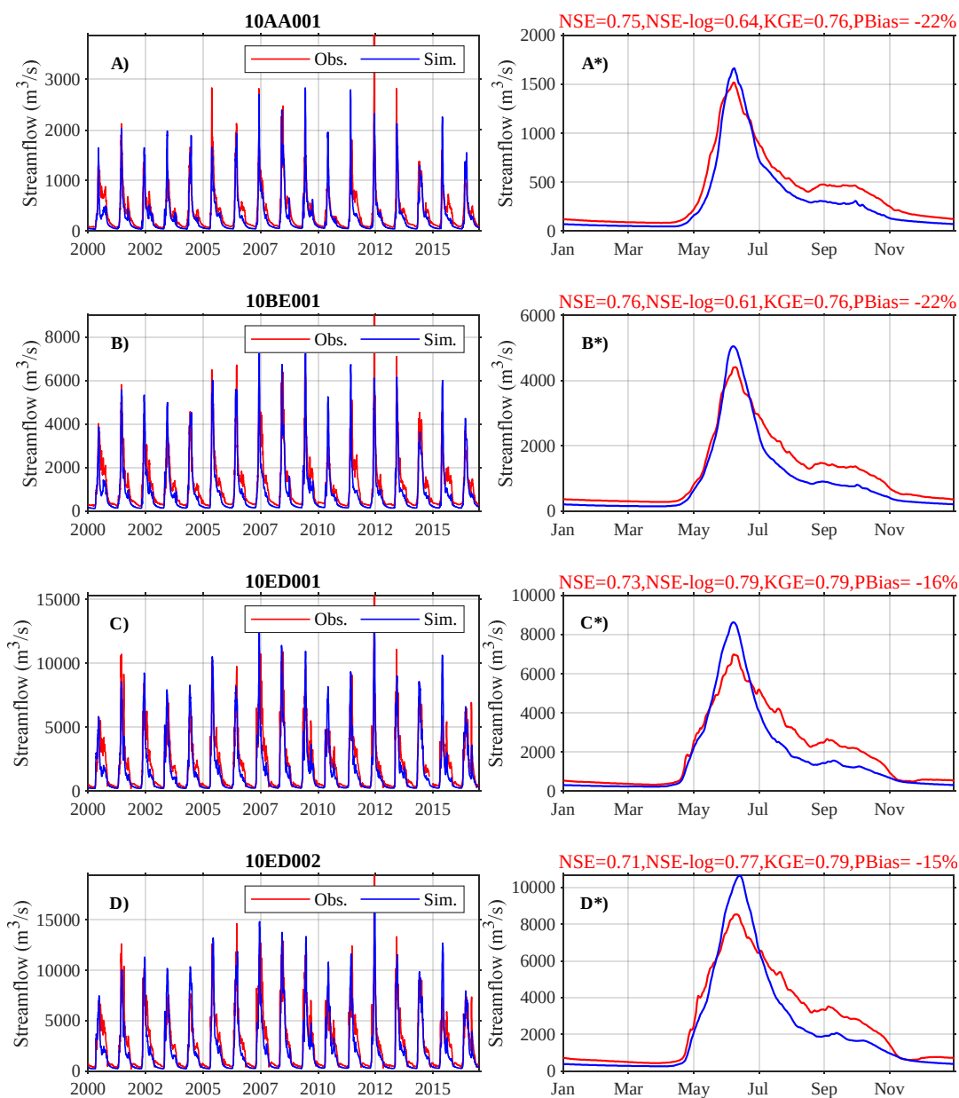
Fig. 10. Daily measured and simulated streamflow for the best performing experiment in terms of streamflow (ID 12) for the 2000-2016 period at four different gauge stations in the LRB: A) 10AA001 (headwaters), B) 10BE001 (intermediate), C) 10ED001 (intermediate), and D) 10ED002 (LRB outlet). For each station, the long-term mean daily hydrograph over the year is provided in a separate subplot with (*) designation, along with performance metrics (in red font).
