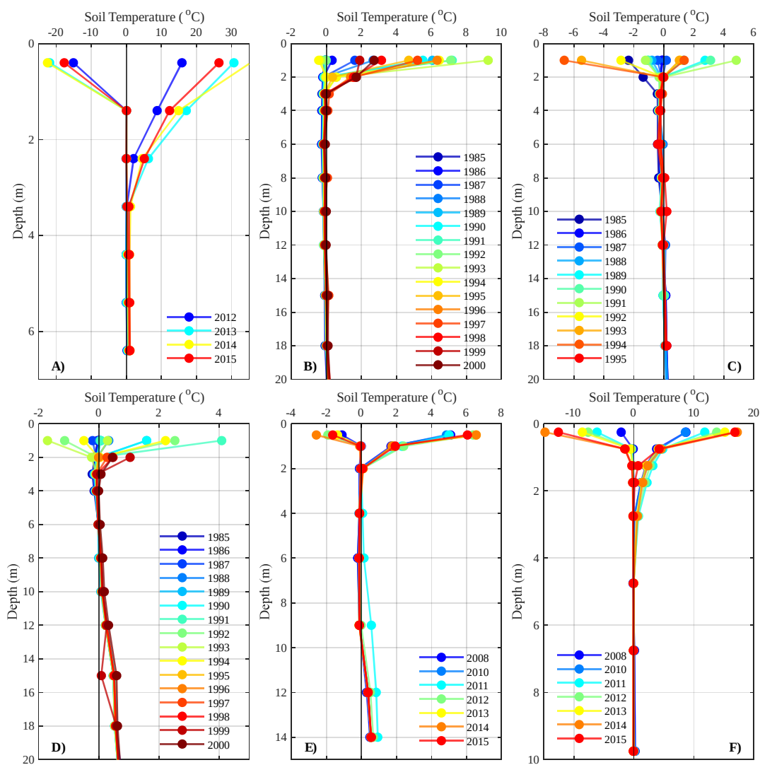
Fig. 3. Observed temperature envelopes at A) Scotty Creek (Fen), B) Petitot River North (84-5A-T4), C) Petitot River North (84-5B-T4), D) Petitot River South (84-6-T6), E) Wrigley Highway (99TC03), and F) Liard Spruce (97TC04) sites.
