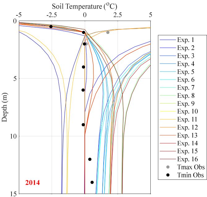
Fig. 6. Observed and simulated temperature profiles at the Wrigley Highway site for the shrubs GRU for the 16 model experiments. The profiles correspond to the same year (2014) for all of the experiments.
